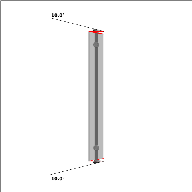
DRAWING 3, Pos 5 SIDE 1, bar length: 335.8 mm
